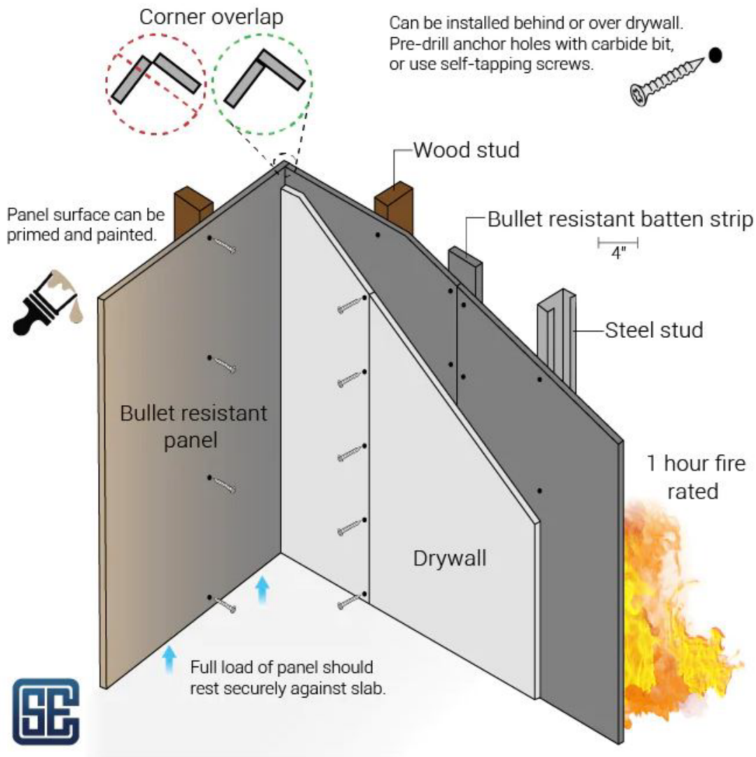
Figure 45: Armortex Installation Diagram, Accessed May 23, 2023
